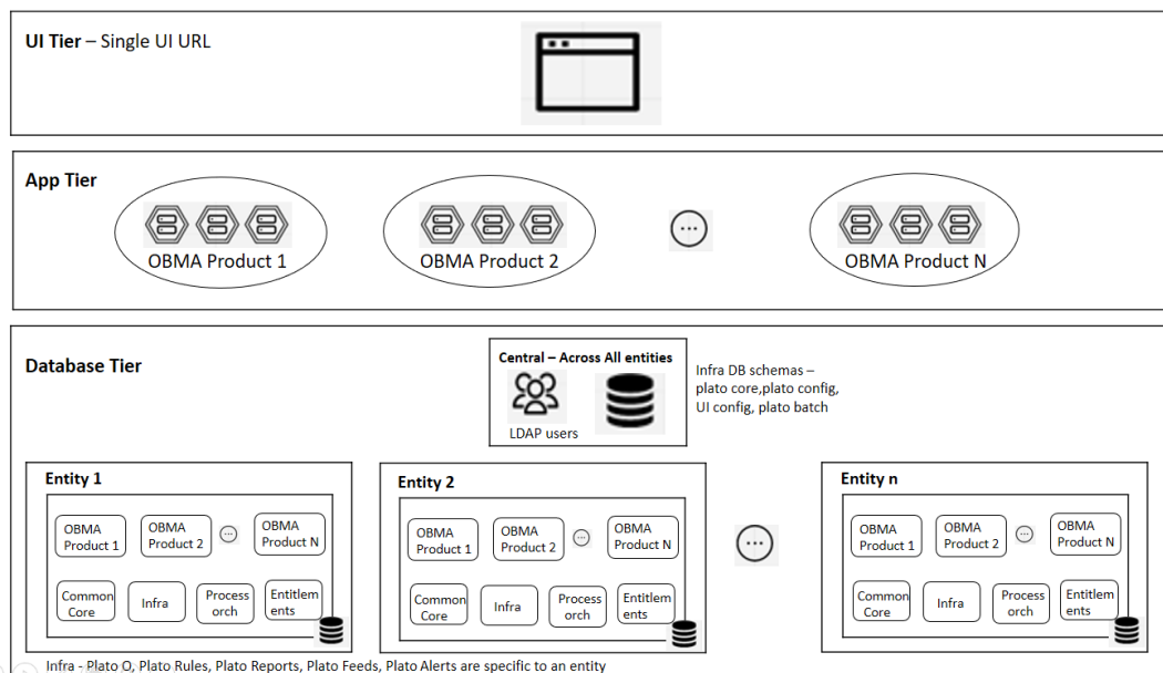
Figure 1: Deployment Diagram.
